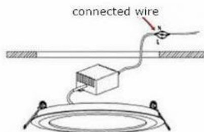
2. Cut off power, the driver wire connected with ceiling wire.
