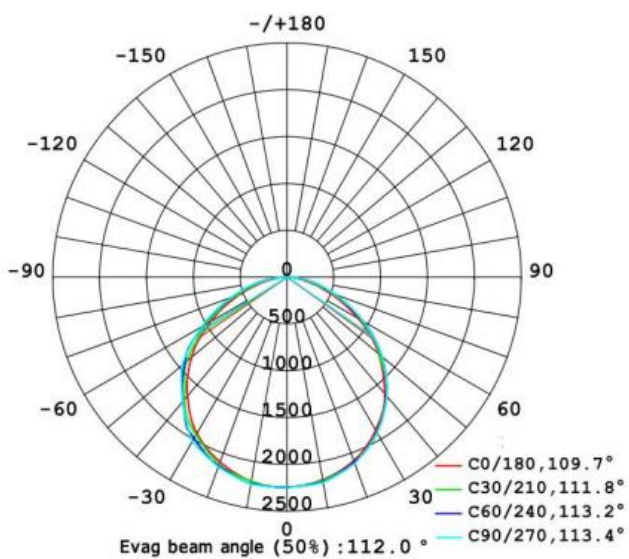
Light Distribution Diagram
