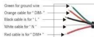
④ Connect with wires and power on
