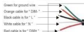
④ Connect with wires and power on
